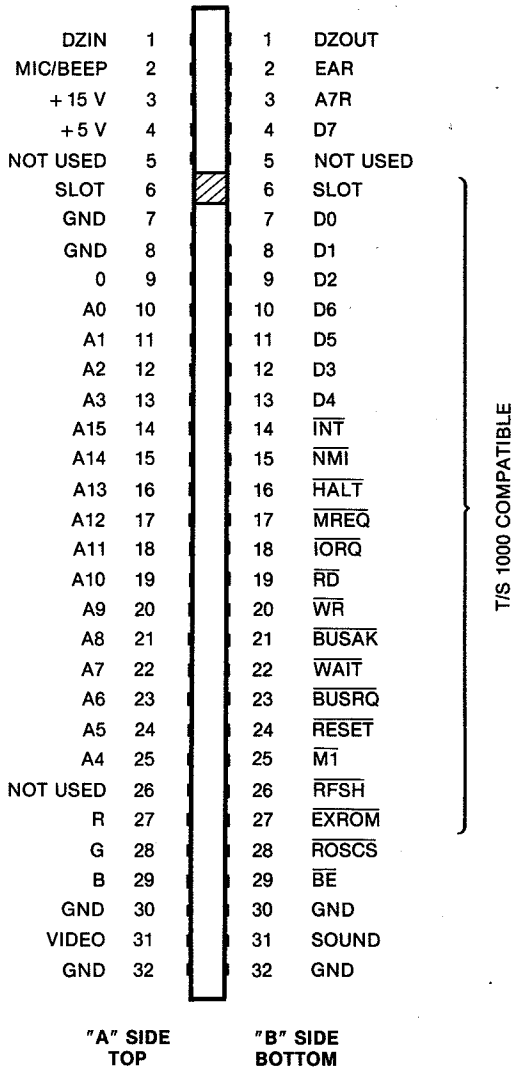
Fig. 6-3. Expansion edge connector.
